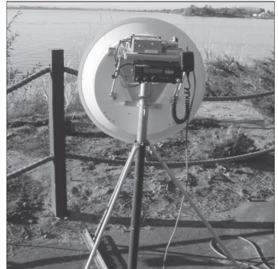
Figure 4.14 — N7CFO's dish antenna operates on 10 GHz and is portable enough to be taken on contest outings.
