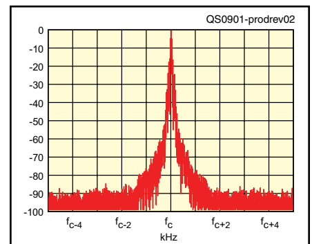
Figure 2 — Spectral display of the K3/100 transmitter during keying sideband testing. Equivalent keying speed is 60 WPM using external keying. Spectrum analyzer resolution bandwidth is 10 Hz, and the sweep time is 30 seconds. The transmitter was being operated at 100 W PEP output on the 14 MHz band, and this plot shows the transmitter output \pm 5\ \text{kHz} from the carrier. The reference level is 0 dBc, and the vertical scale is in dB.
