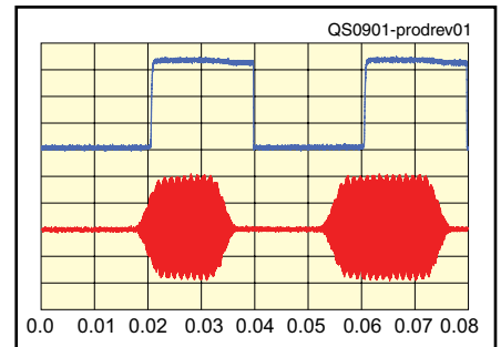
Figure 1 — CW keying waveform for the K3/100 showing the first two dits in full-break-in (QSK) mode using external keying. Equivalent keying speed is 60 WPM. The upper trace is the actual key closure; the lower trace is the RF envelope. (Note that the first key closure starts at the left edge of the figure.) Horizontal divisions are 10 ms. The transceiver was being operated at 100 W output on the 14 MHz band.
