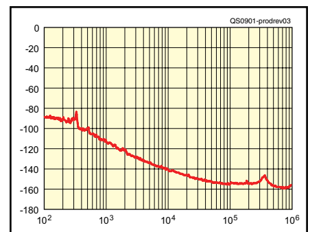
Figure 3 — Spectral display of the K3/100 transmitter output during composite-noise testing. Power output is 100 W on the 14 MHz band. The carrier, off the left edge of the plot, is not shown. This plot shows composite transmitted noise 100 Hz to 1 MHz from the carrier. The reference level is 0 dBc, and the vertical scale is in dB.
