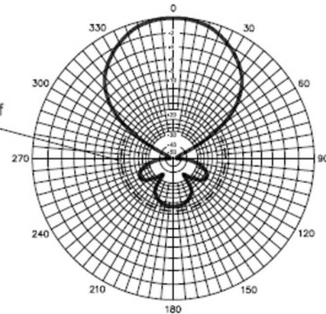
Radiation Pattern
